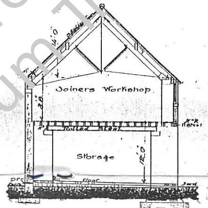
Section thro' Workshop etc
